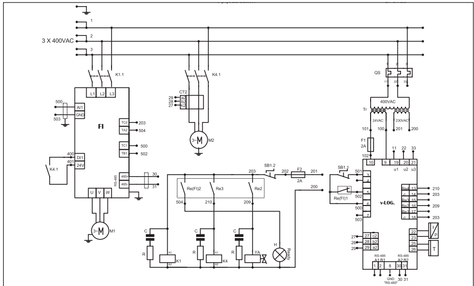
Fig. 2.6 Electrical diagram FV30-55
